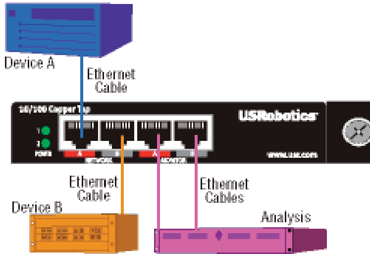
Simple Tap Connection Diagram
